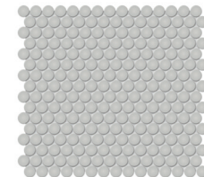
3/4 in / 1.9 cm Penny Round Mosaic Actual: 289 x 313 x 6 mm Glossy 4501-0430-0 Matte 4501-0439-0
