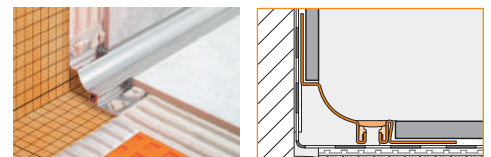
4.15 Schluter®-DILEX-HKS
