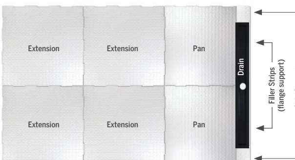
END DRAIN WITH PROVA LINEAR PAN EXTENSION® KIT - 4' X 6' (122 cm x 183 cm)
