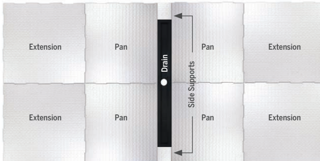
CENTER DRAIN WITH PROVA LINEAR PAN EXTENSION® KIT - 4' X 8' (122 cm x 244 cm)
