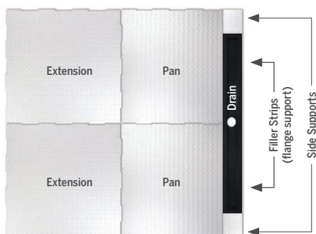
END DRAIN - 4' X 4' (122 cm x 122 cm)
