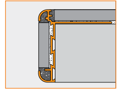
2.9 Schluter®-RODEC-CT
