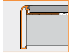
2.8 Schluter®-RODEC-STEP
