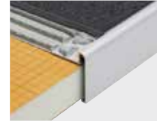
2.8 Schluter®-RODEC-STEP
