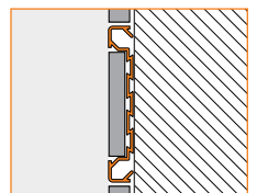
2.11 Schluter®-QUADEC-FS
