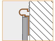
2.5 Schluter®-RODEC-DB
