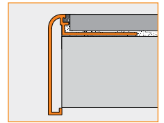
2.8 Schluter®-RONDEC-STEP
