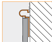
2.5 Schluter®-RONDEC-DB
