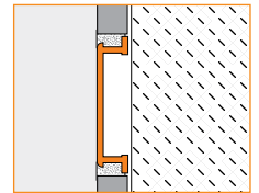
2.2 Schluter®-DESIGNLINE
