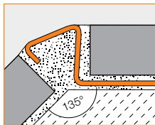
2.14 Schluter®-DECO-DE
