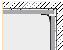
2.7 Schluter®-ECK-KHK
