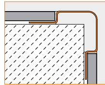
2.13 Schluter®-DIADEC
