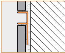
1.9 Schluter®-DECO-SG
