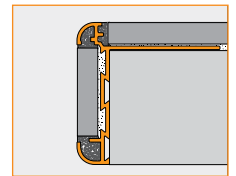
2.9 Schluter®-RONDEC-CT
