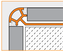
2.10 Schluter®-QUADEC
