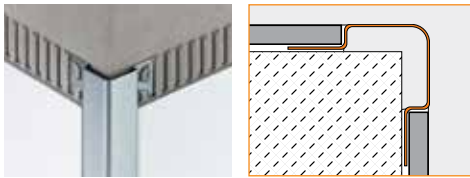
2.6 Schluter®-ECK-E
