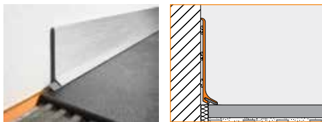
16.2 Schluter®-DESIGNBASE-SL
