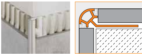
2.1 Schluter®-RONDEC
