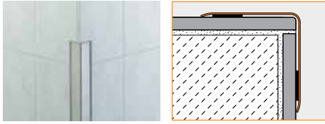
2.7 Schluter®-ECK-K
