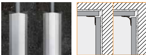
2.7 Schluter®-ECK-KI/-KHK
