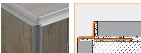
2.12 Schluter®-INDEC
