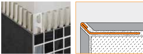
2.17 Schluter®-FINEC
