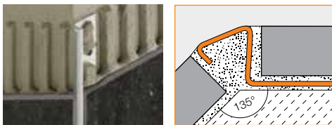
2.14 Schluter®-DECO-DE
