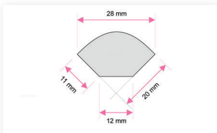
Vinyl Quarter-Round
