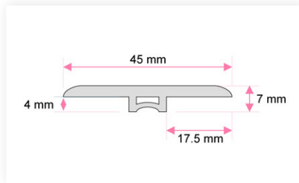
Vinyl T-Molding
