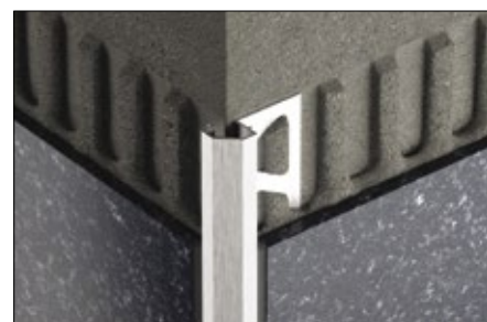
Outside corner 90°
