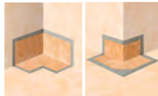
Schluter®-KERDI-KERECK-F Page 112
