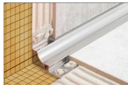
Inside corner, 2-way (90°)
