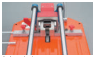
Single-point breaker.
