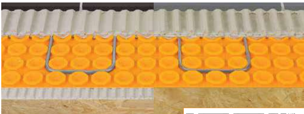
6.4 Schluter®-DITRA-HEAT/PS
