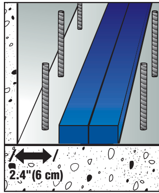
Where two strips of Idrostop are used side by side, 2.4" (6 cm) of concrete is sufficient to protect the gasket.
