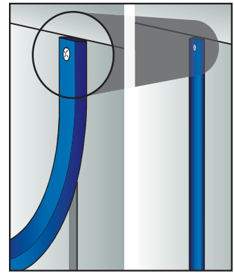
Pieces longer than 3.3 feet (1 m) can be installed on vertical surfaces by fixing the top of the pieces with a nail or pin and then extruding the MS-polymer-based adhesive directly onto the underlying substrate.
