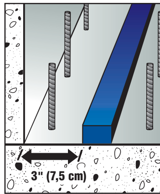
Width of concrete to protect Idrostop
