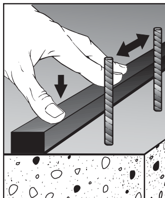
Firmly press Idrostop , moving it in all directions to make it adhere well.
