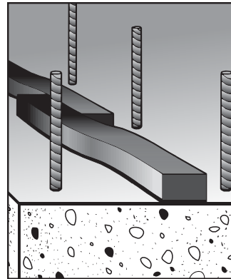
In-line joint: The two ends are staggered with an overlap of 0.8" to 1.2" (2 to 3 cm) for a better seal.
