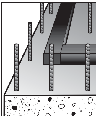
Horizontal corner joint
