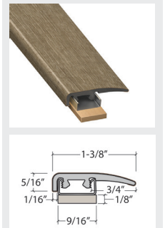
SlimCap with Track and Shim
