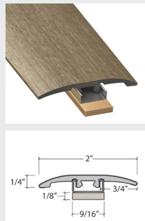
SlimTrim with Track and Shim
