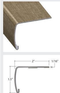
VersaEdge Extra Tall
